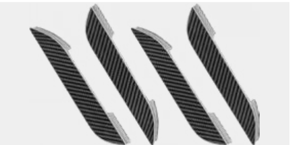
Product: Car Door Handle Cover For Tesla Model S Material: Toray 3K Carbon fibre prepreg Specification: 4Pcs/Set Fitment: 2017 Model S Installation: Paste
