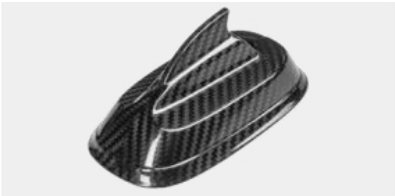
Product: Antenna Cover For BMW MINI-F56 Material: Toray 3K Carbon Fibre Prepreg Specification: 1Pcs/Set Fitment: F54 Low allocation,F55F56F57 Installation: Paste
